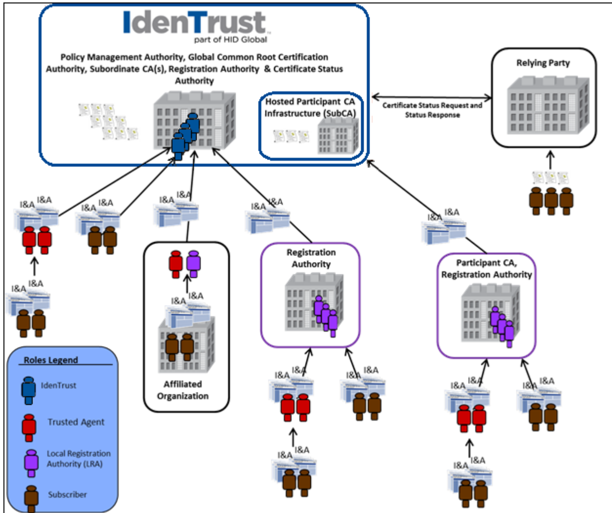
Figure 1: PKI Participants
